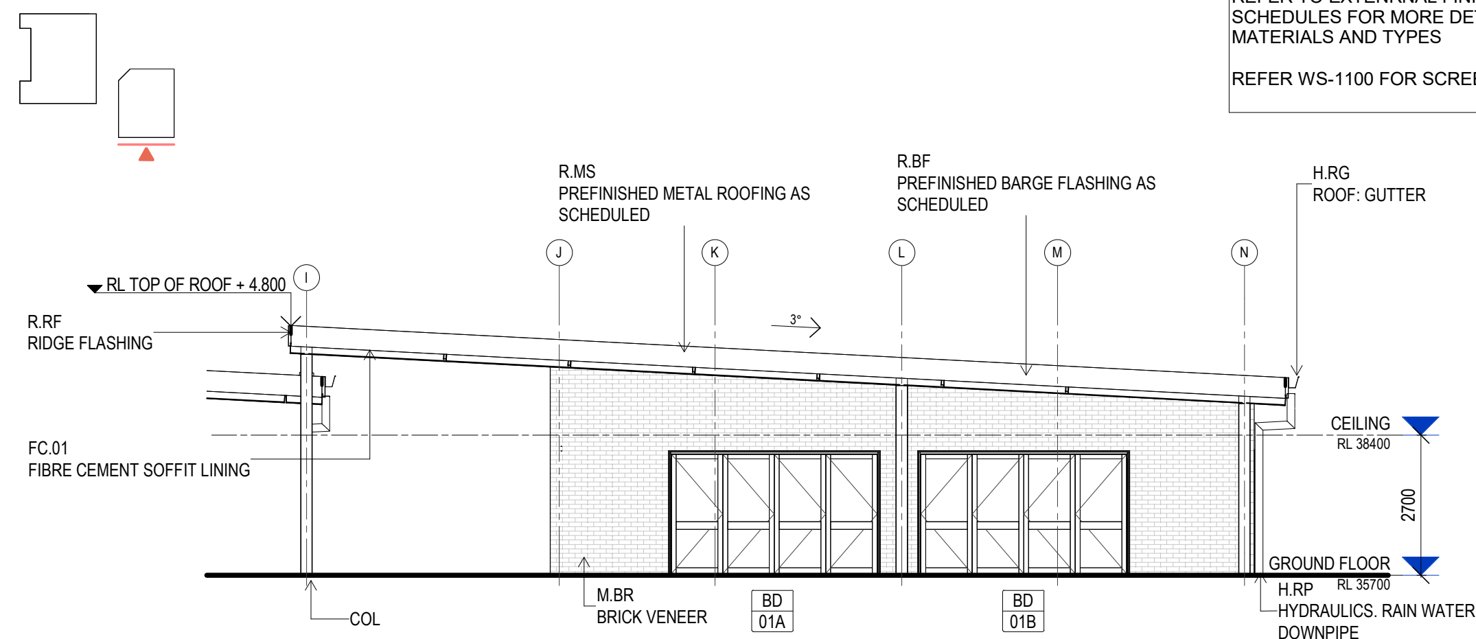
2 ELEVATION SOUTH Scale: 1 : 100
